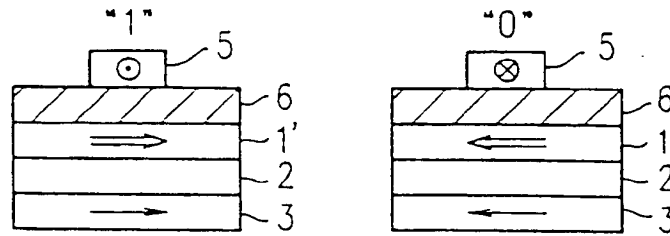
FIG. 6A Information recording by current
